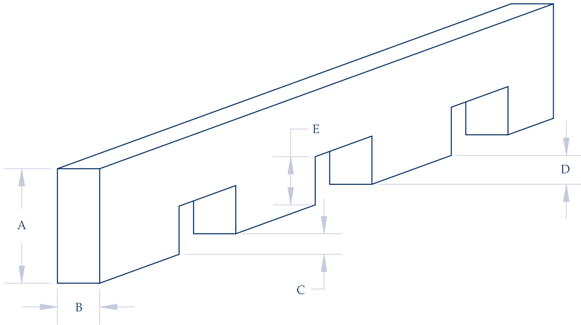
IL DENT 3 Single-Cut Dentil – Under Cut (Dimensions Can Vary)
