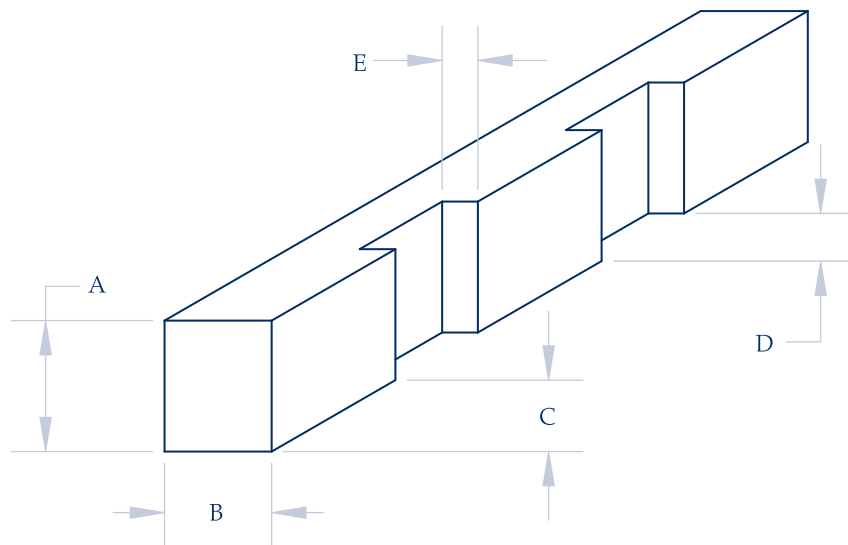
IL DENT 1 Single-Cut Dentil – Face Cut (Dimensions Can Vary)
